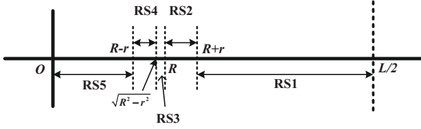
Fig. 1. Division of road segments for computation of cache coverage ratio.
