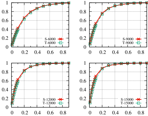
Fig. 2. Comparison between simulations and theoretical analysis with the transmission radius set to 150 m. The x -axis and y -axis represent the caching probability and the one-hop cache coverage ratio respectively. Legend “S-6000” and “T-6000” denote the result for simulation and theoretical analysis with a total vehicle number of 6,000 respectively, similar for others.
