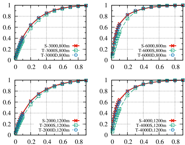
Fig. 5. Results for different street lengths. The x -axis and y -axis represent the caching probability and the one-hop cache coverage ratio respectively. Legend “S-3000,800m” denotes the simulation result with 3,000 vehicles and the street length of 800 m, while “T-3000S,800m” and “T-3000D,800m” denote the theoretical result using the same and different rate parameters respectively, similar for others.
