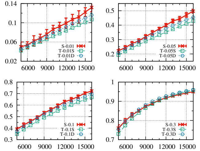
Fig. 3. Comparison between simulations and theoretical analysis with the transmission radius set to 150 m. The x -axis and y -axis represent the total vehicle number and the one-hop cache coverage ratio respectively, and the error bars represent the standard derivation in simulation. Legend “S-0.1” denotes the simulation result with the caching probability of 0.1, while “T-0.1S” and “T-0.1D” denote the theoretical result using the same and different rate parameters respectively, similar for others.
